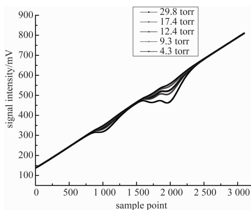
图 4 室温下不同压强下的探测信号 Fig. 4 Detection signals under different pressures at room temperature
