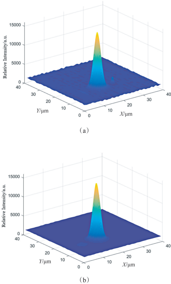
Fig. 10 Spot comparison before and after correction: (a) original spot; (b) corrected spot 图 10 矫正前后光斑对比: (a) 原始光斑; (b) 矫正后光斑
