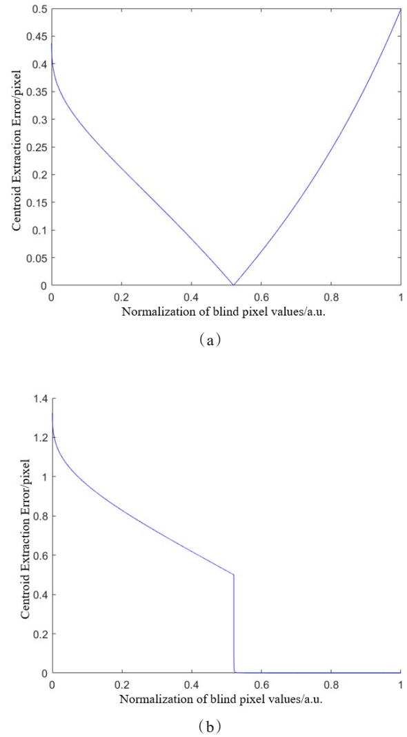
Fig. 11 Influence of the blind pixel on the spot centroid localization accuracy: (a) 1 pixel from the center of the spot; (b) the blind pixel is located at the center pixel of the spot 图 11 盲元对光斑质心定位精度的影响: (a) 距光斑质心一个像素点; (b) 盲元位于光斑质心像素点
